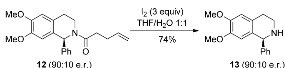
Scheme 2. Cleavage of the pent-4-enoyl without racemization.
