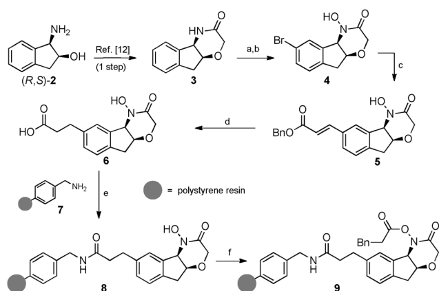
Scheme 1. Preparation of solid-supported amine-resolving agent 9 . Reagents and conditions: a) TFA/H 2 SO 4 (3:1) 0°C, then NBS (1.01 equiv), 80%; b) N,O-bis(trimethylsilyl)acetamide (1.1 equiv), CH 3 CN, 23°C to 75°C, then MoO 5 ·Py·HMPA (MoOPH) (1.2 equiv), CH 2 Cl 2 , 23°C, 73%; c) benzylacrylate (1.50 equiv), Pd(OAc) 2 (0.10 equiv), P( o -tolyl) 3 (0.21 equiv), Et 3 N (5.00 equiv), CH 3 CN, 23°C to 75°C, 65%; d) Ac 2 O (1.10 equiv), EtOAc, 23°C to 45°C, then Pd/C (10 wt%), H 2 ; then 1 M LiOH, 73%; e) 7 (0.50 equiv), HATU (0.95 equiv), DMAP (1.00 equiv), Hünig's base (3.00 equiv), DMF; f) 3-phenylpropanoic anhydride, DMF, 45°C. Abbreviations: TFA = trifluoroacetic acid, NBS = N -bromosuccinimide, Py = pyridine, HMPA = hexamethylphosphoric acid triamide, HATU = 2-(1 H -7-azabenzotriazol-1-yl)-1,1,3,3-tetramethyl uronium hexafluorophosphate, DMAP = 4-dimethylaminopyridine.
