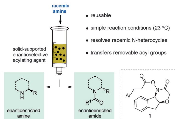
Figure 1. Kinetic resolution of N-heterocycles with a reusable, solid-supported reagent based on chiral stoichiometric reagent 1 .
